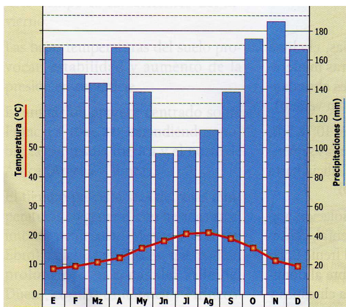
Climograma 1
