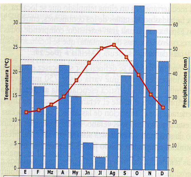
Climograma 2
